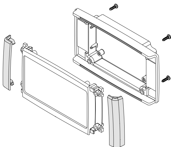
Mounting frame for wall fitting
