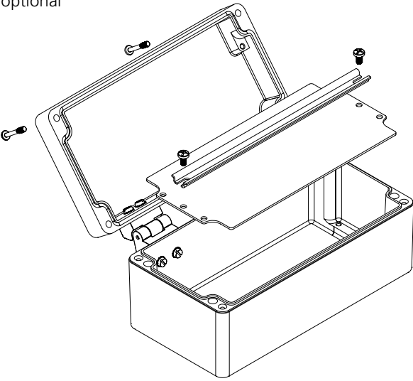
Variant with hinge optional
