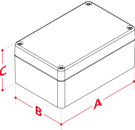
Variant with hinge optional
