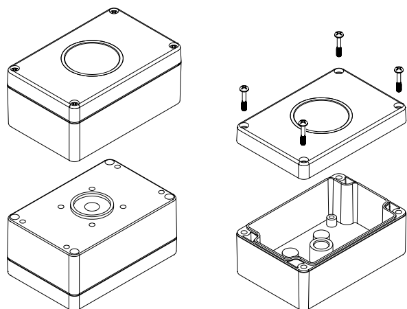
V 215 F05 Variant with F05 holder
