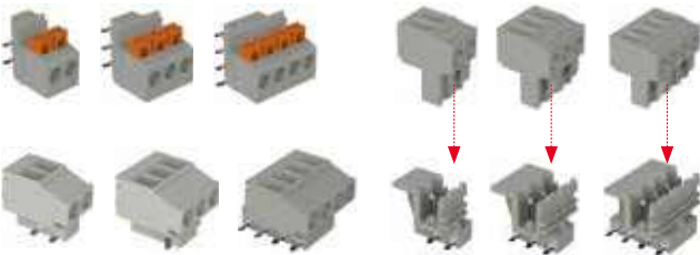
Screw connection terminal blocks, single / double section and spring-cage terminal blocks, single section
