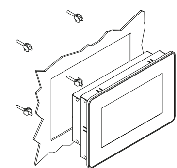
Control panel mounting
