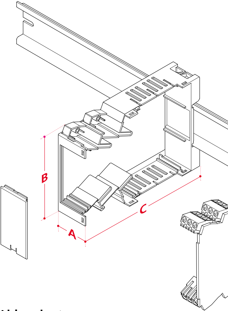
CN-DU for rectangular PCBs
