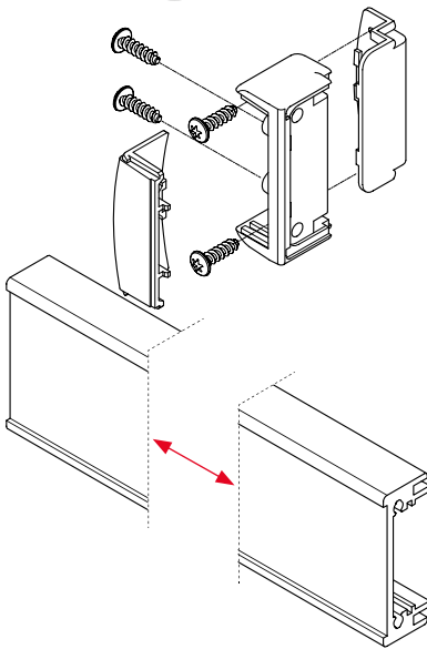
Frontplatte screwable, only with AP 10...
